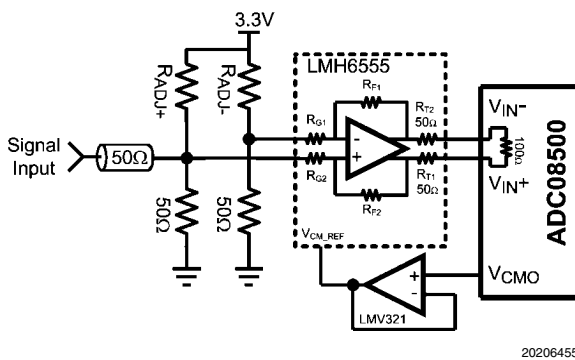
FIGURE 13. Example of Servicing the Analog Input with V_{CMO}
